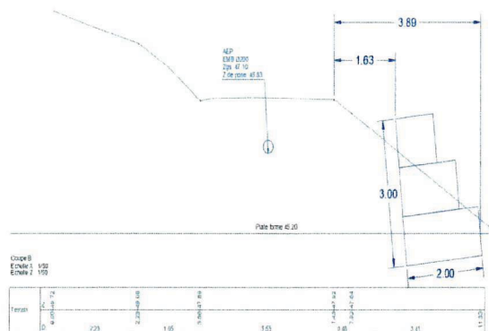
Figure 2 - Coupe B
