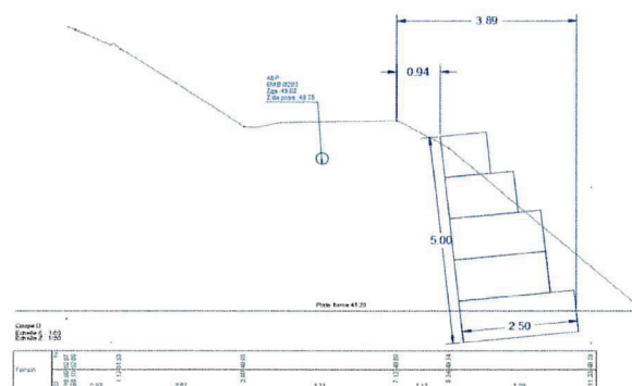
Figure 4 - Coupe D
