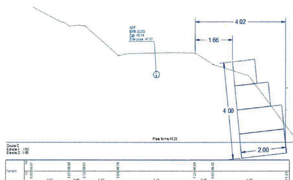
Figure 3 - Coupe C
